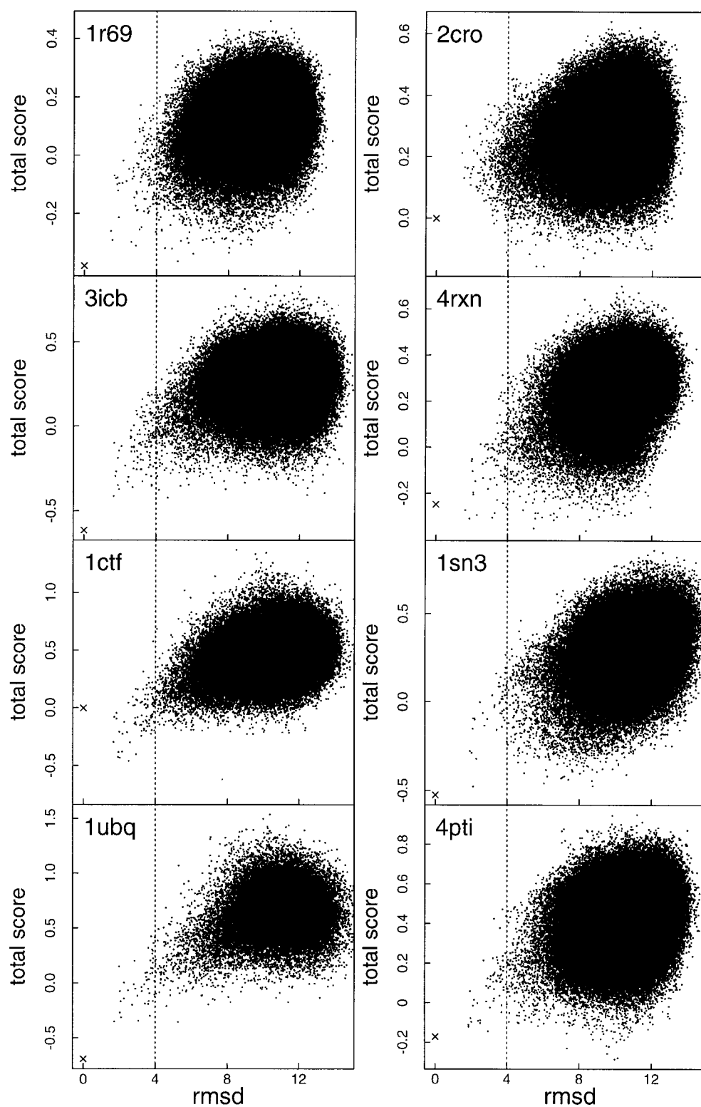
Fig. 7. Plots of -\log P(\text{structure}|\text{sequence}) vs rmsd for the eight decoy sets of Park and Levitt. 11 Native-like structures ( <4 \text{ \AA} rmsd) are distinguished from the ensemble of non-native structures for most of the proteins.
