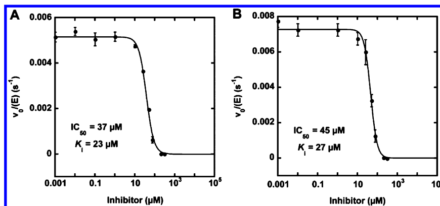
Figure 5. Inhibition of a FR29 and a ECH19 variant by tyrosyl ester 1. The IC_{50} of tyrosyl ester 1 was determined by incubating (A) FR29 A44S/T112L/V151L ( [E] = 2 \mu M ) and (B) ECH19 K354P/P364W ( [E] = 2 \mu M ) with increasing amounts of the inhibitor ( [I] = 0.001\text{--}300 \mu M ) before 50 \mu M of coumarin ester 2 was added and the release of coumarin was monitored. The IC_{50} was determined by curve fitting and converted into the corresponding K_i using the Cheng–Prusoff equation. 37
